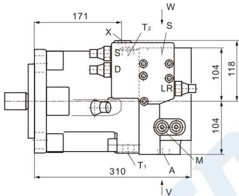
With change pump Detail W
