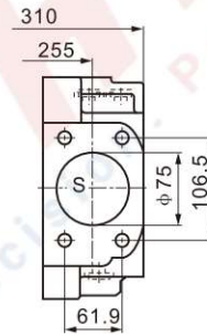
Without change pump Detail W
