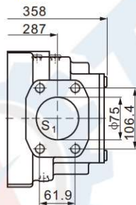
With change pump Detail W
