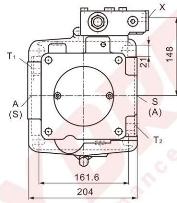
Without change pump Detail W
