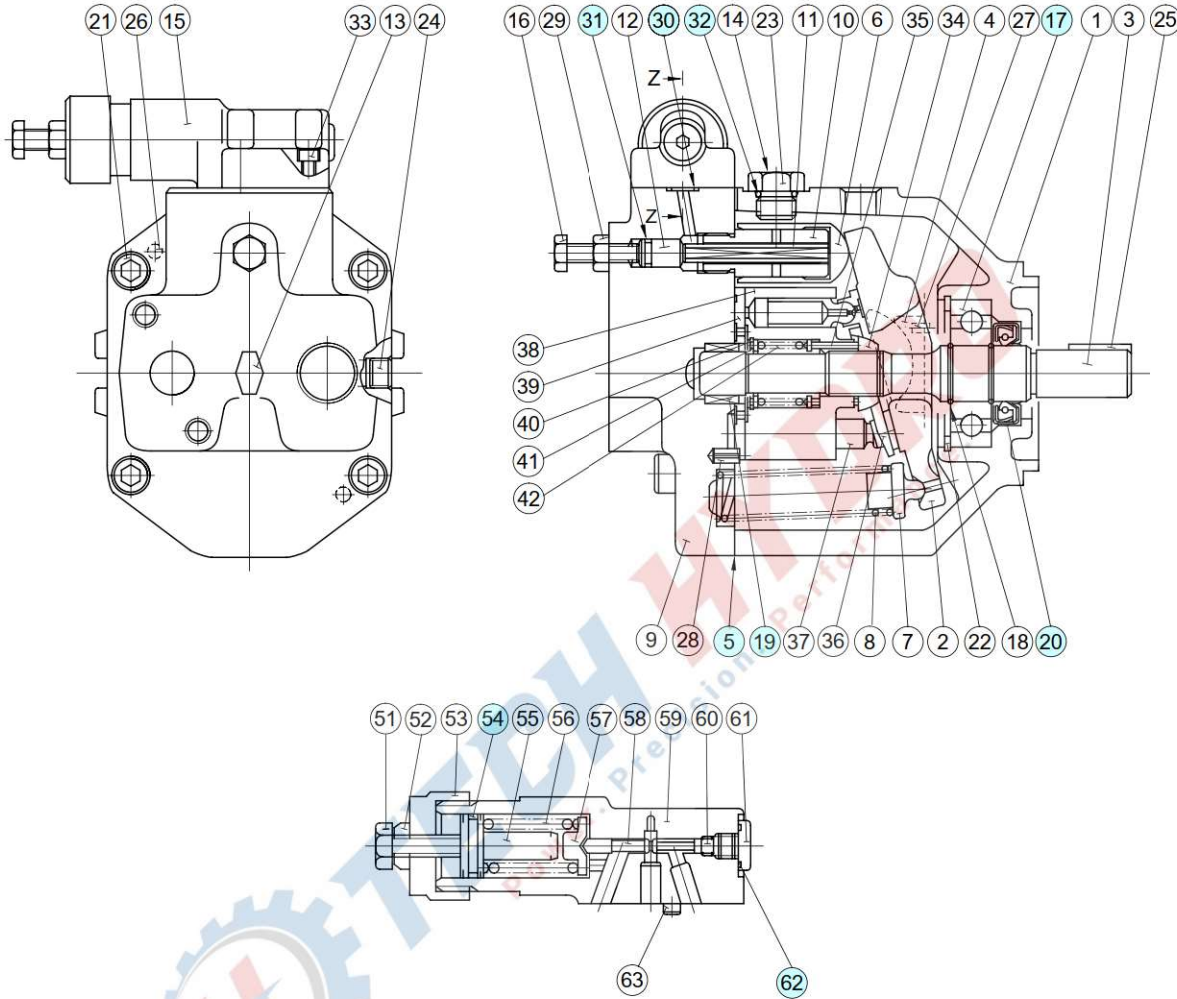
Section Z-Z
