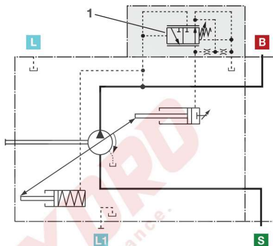
1. Pressure controller - DR
