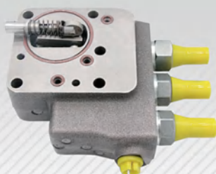
A29 LRDS Valve TYPE : A11VO190/260 MODEL: 4KG
