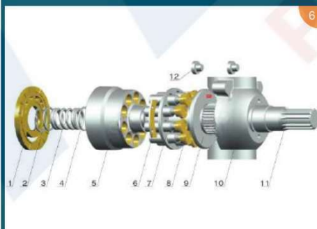
CAT12G/14G/16G
