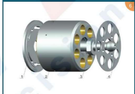
BMF50/75/105
