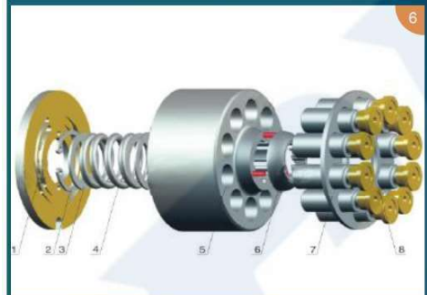
A10VE43/A10VEC60
