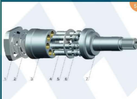
BPR140/186/260
