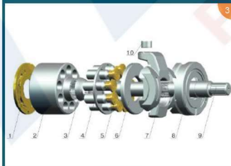
K3VL45/80
