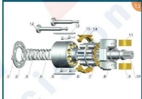
HMF160/200
