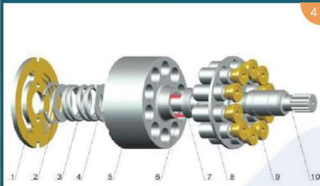
KYB-25CC/IHISCE 60/PSVK2-25
