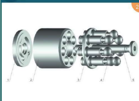
B2PV35~140
