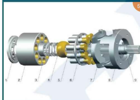
NV64/NV84/NV111DT/NV137/NV172/NV270
