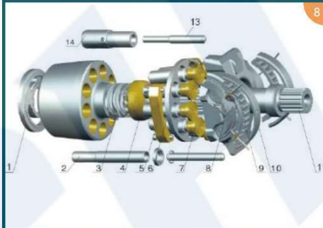
A11VO40/60/75/95/200/250/A11VG35/50/A11V130~190/ A11VLO190/260
