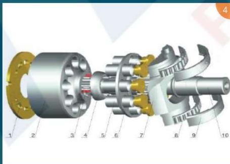
A10VG18~63
