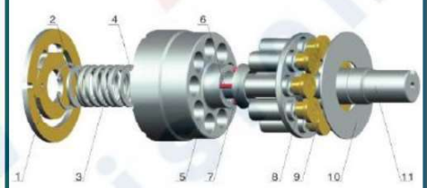
PV29/PV74
