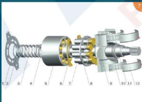
PV90R030~250
