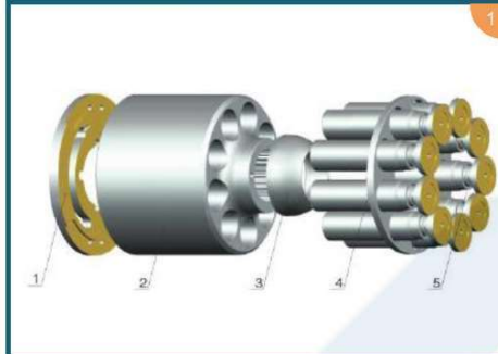
HAWE V60A
