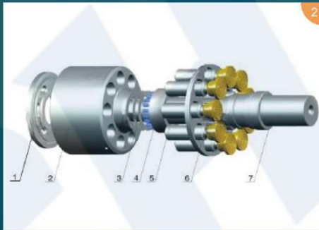
A4VF500/A4VG28~71/A4VTG71/A4VG90~250/A4VHW90
