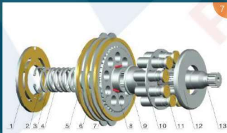
MSG-27P(KYB)/(LSGMF27/10W)/MSG-44P(KYB)/LSGMF44/10W-R21
