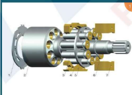
HPV55T(LINDE)/HPR75/100/105/130/LINDE HMR135/HPR
