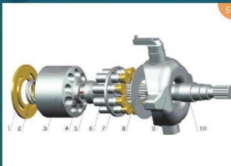
A10V43/63/A10VD40/43
