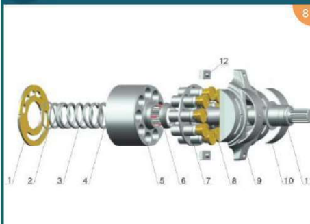
BRL100
