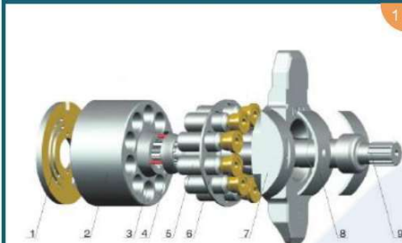
PVD-2B-32L/34L/36L/38/40/42/63
