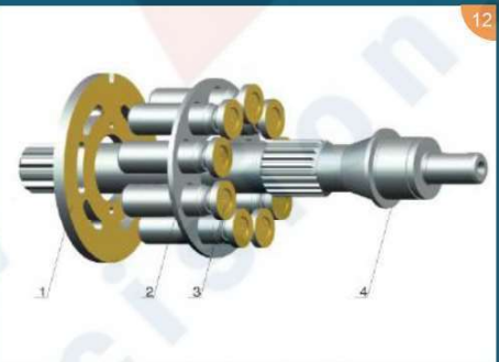
HPVMF23(T23C)/HPVMF23.7/T28C/T30C/T37C
