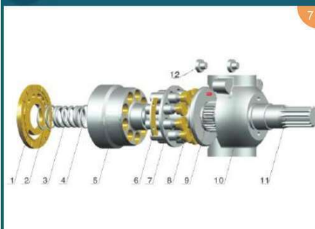
CAT215/245/992
