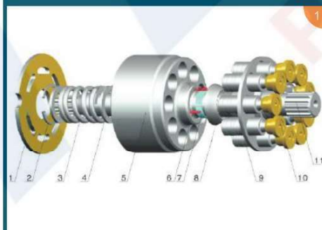
EATON 006/3322/3932-243/4621/4631-007/5421/5431/6423/7621/78462/CASE1460
