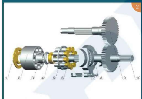
SBS80(CAT312C)
