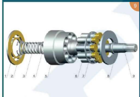
SPV14/SPV15/SPV18/MMFO25C
